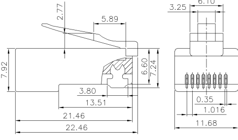
RECOMMENDED 8P PLUG TOLERANCE ±0.05
