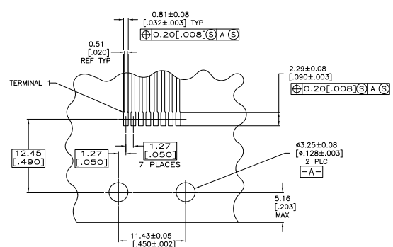
RECOMMENDED PRINTED CIRCUIT BOARD LAYOUT COMPONENT SIDE
