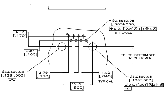
SUGGESTED PRINTED CIRCUIT BOARD LAYOUT (COMPONENT SIDE)
