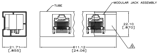
DETAIL A TUBE PACKAGING SCALE 2:1
