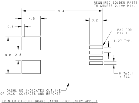
PRINTED CIRCUIT BOARD LAYOUT (TOP ENTRY APPL.)
