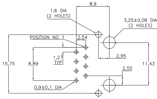
PRINTED CIRCUIT BOARD LAYOUT [VIEW SHOWN IS CIRCUIT (NONCOMPONENT) SIDE OF BOARD.] TOLERANCES UNLESS OTHERWISE SPECIFIED: ± 0.05 PRINTED CIRCUIT BOARD THICKNESS: 1,6 mm NOMINAL.
