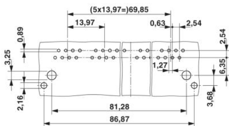
Drilling plan/solder pad geometry
