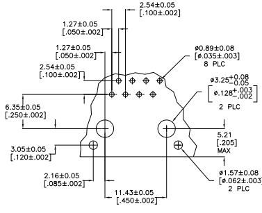
RECOMMENDED PRINTED CIRCUIT BOARD LAYOUT (COMPONENT SIDE)
