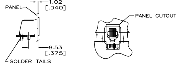
RECOMMENDED PANEL CUTOUT GUIDELINES SCALE 1:1
