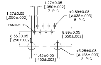
RECOMMENDED PRINTED CIRCUIT BOARD LAYOUT COMPONENT SIDE SCALE 4:1
