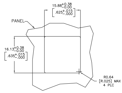
RECOMMENDED PANEL CUTOUT SCALE 4:1
