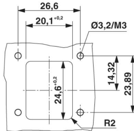
Panel cutout
