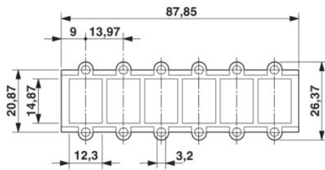
RJ45 panel mounting frame, IP20
