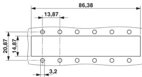
Panel cutout
