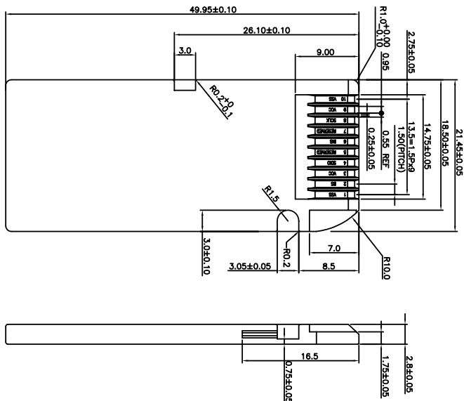
RECOMMENDED CARD LAYOUT
