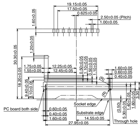
Recommended PC board pattern (TOP VIEW)
