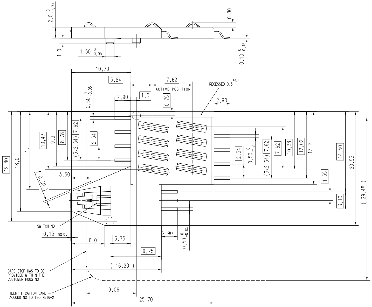
PCB - LAYOUT
