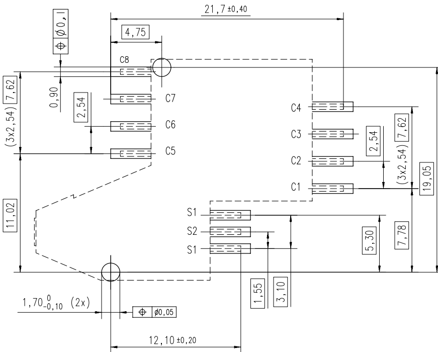
PCB - LAYOUT
