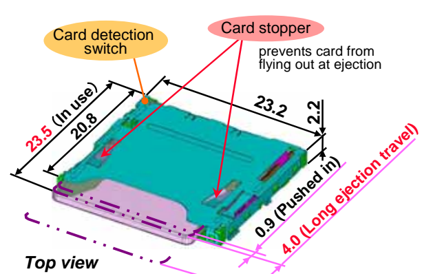
DM2A (Top mount type)
