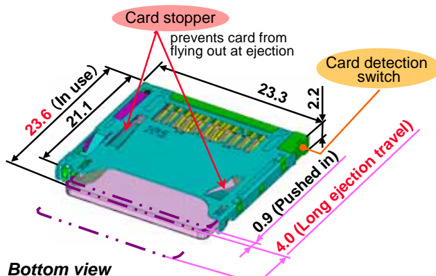
DM2B (Bottom mount type)
