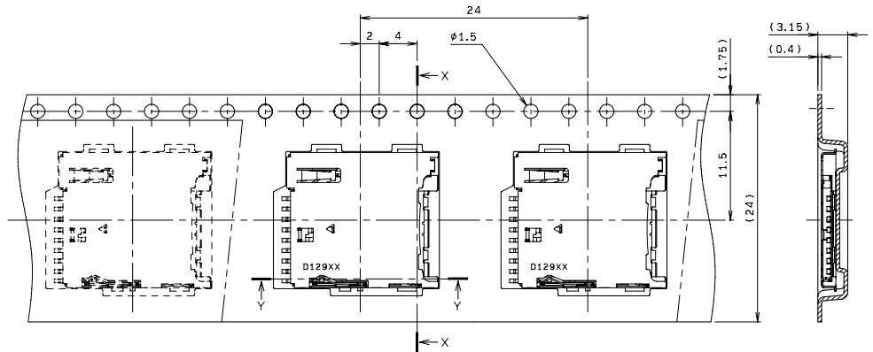
SECT. X-X
