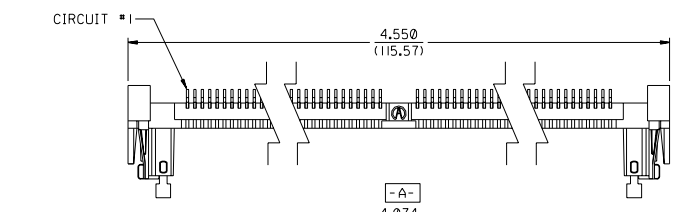
"SIMM" P.C. BOARD LAYOUT
