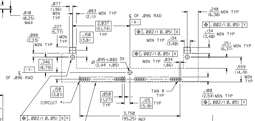
RECOMMENDED SOCKET P.C. BOARD PAD PATTERN
