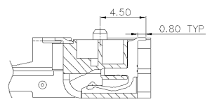
SEC B-B SCALE 2:1
