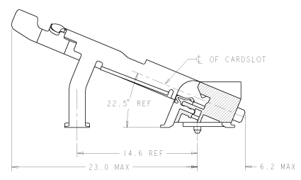
SECTION P-P SCALE 6:1
