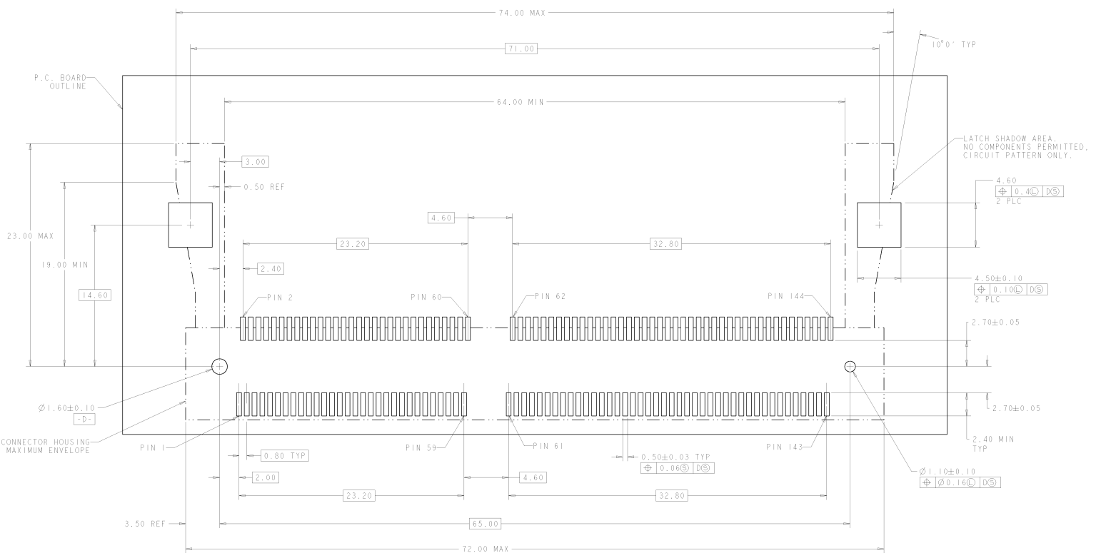
RECOMMENDED MOTHERBOARD FOOTPRINT SCALE 7:1
