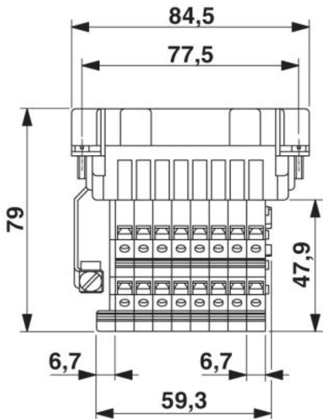
Dimensioned drawing
