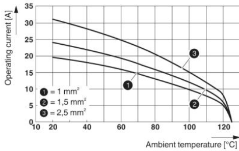
Derating diagram: Series HC-A 3-E..S / HC-A 4-E..S
