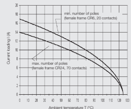
ConCept module CM-10 Conductor H07V-K 2.5 mm 2
