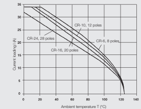
ConCept module CM-HE Conductor H07V-K 4.0 mm 2
