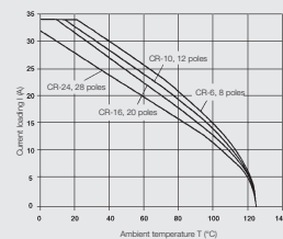
ConCept module CM-HE Conductor H07V-K 4.0 mm 2
