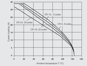
ConCept module CM-HE Conductor H07V-K 4.0 mm 2
