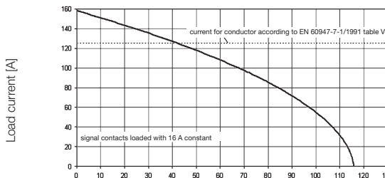
HDC-S6/6-SAS/BAS Ambient temperature [°C] power contacts H07V-K35
