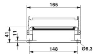
Dimensional drawing
