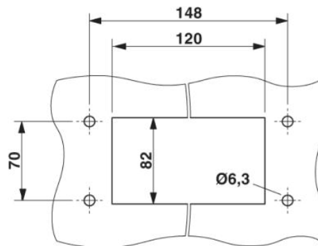
Panel cutout
