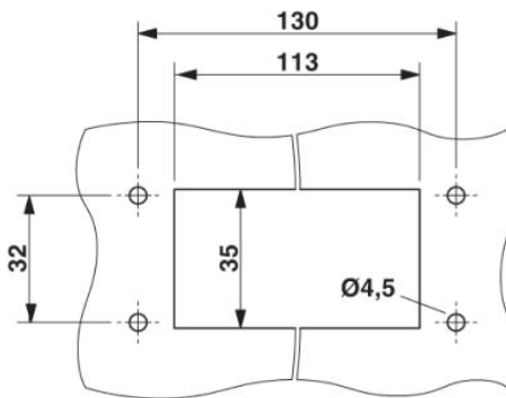
Panel cutout
