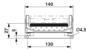
Dimensional drawing
