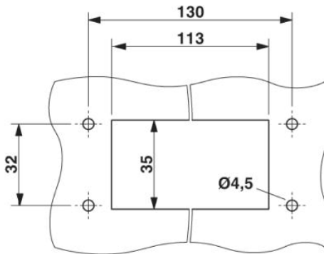
Panel cutout
