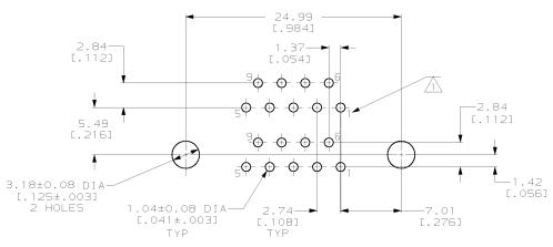
RECOMMENDED PC BOARD MOUNTING DIMENSIONS 1.57(.062) PC BOARD THICKNESS
