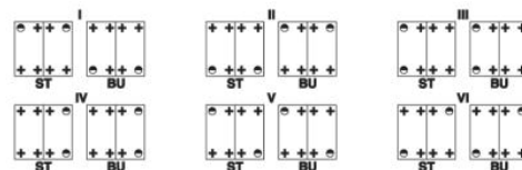
Coding for housings with two contact inserts
