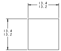
RECOMMENDED PANEL CUTOUT MAX PANEL THK. 1.7
