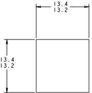
RECOMMENDED PANEL CUTOUT MAX PANEL THK. 1.7
