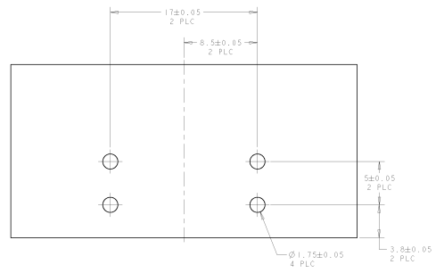
SUGGESTED HOLE PATTERN SCALE 5:1
