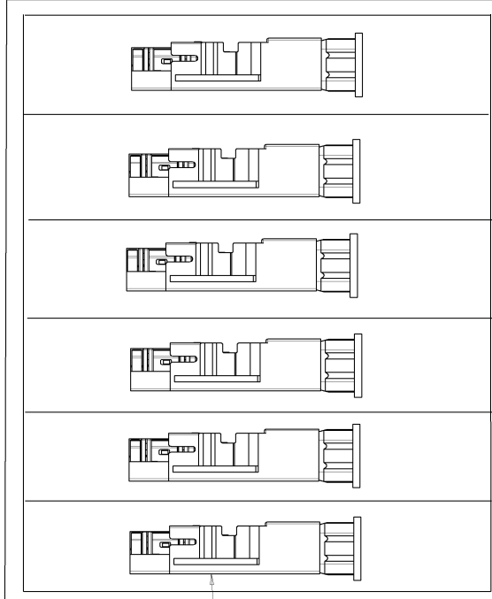
MT-RJ SECURE 250um JACK MODULE ASSEMBLY
