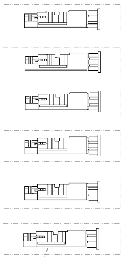
MT-RJ SECURE JACK-XG MODULE ASSEMBLY
