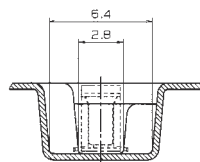
SECT. F-F
