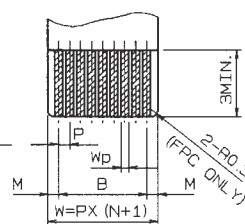
SUPPORTING TAPE
