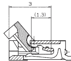
SECT. X-X
