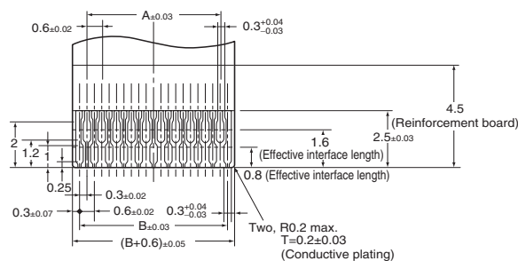
Applicable FPC Dimensions
