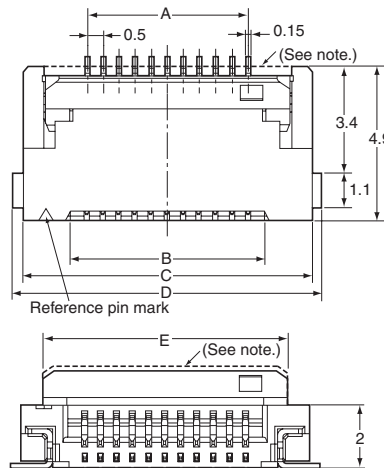
PCB Mating Dimensions (Top View)
