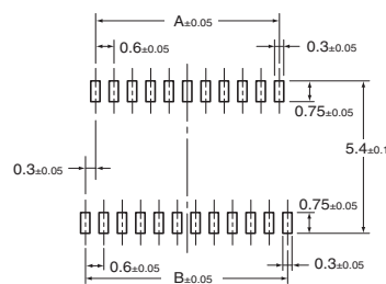
PCB Mating Dimensions (Top View)
