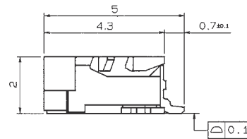
SECT X-X
