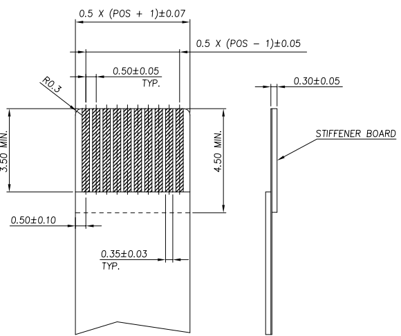
RECOMMENDED FPC DIMENSIONS DIAGRAM
