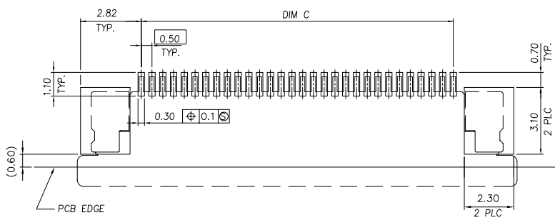
RECOMMENDED PCB DIMENSIONS DIAGRAM TOLERANCE: ±0.05
