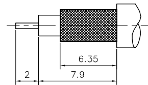
Trim cable
