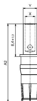
Power crimp contact (short version)
