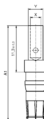
Power crimp contact (standard version)
