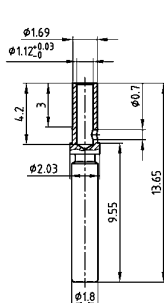
Signal crimp contact (closed entry version)
