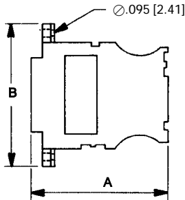
Junction Shell
