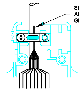
ITEM No. 1, 3, 4 & 5 TOP ENTRY
