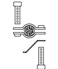
STRAIN RELIEF AND GROUNDING SPRING MOUNTING DETAIL
