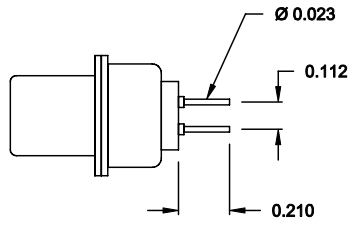
SIGNAL CONTACTS
