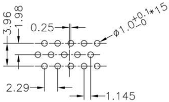
15 Pin Male Connector PCB Pin Layout Scale 2:1
