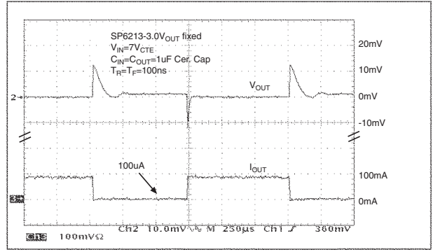
Load Transient Response ( V_{IN} = 7V )
