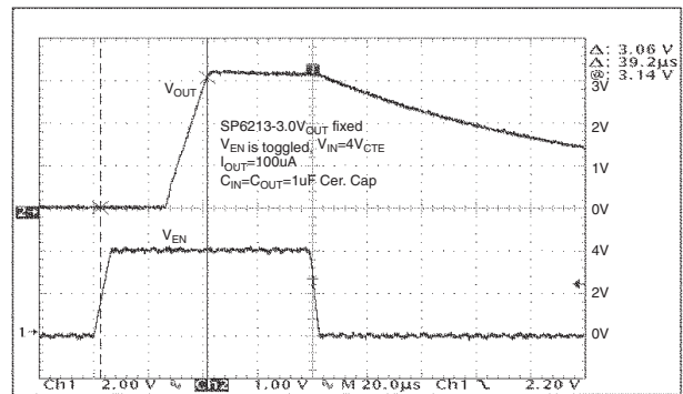
Turn-on Characteristic ( V_{IN} = 4V , I_{OUT} = 100\mu A )
