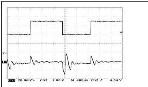
Line Transient Response ( V_{IN}=7V , I_{OUT}=100\mu A )
