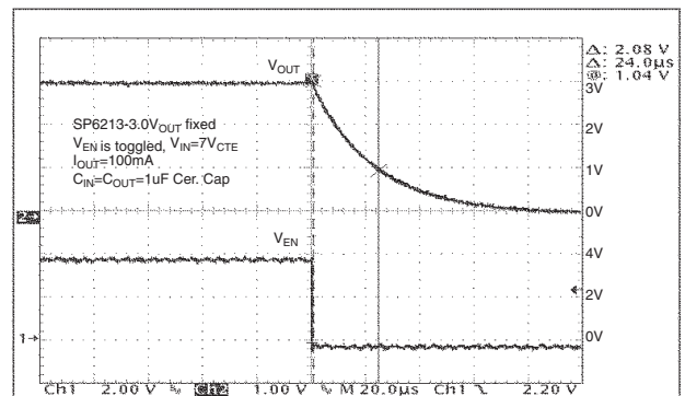
Turn off Time ( V_{IN} = 7V , I_{OUT} = 100mA )
