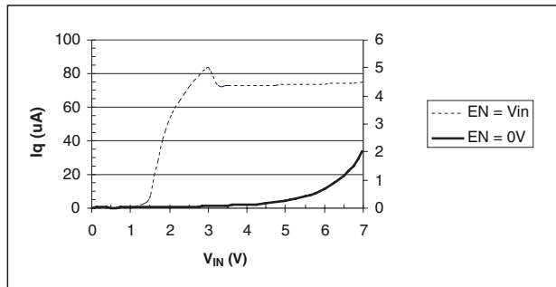
Quiescent Current vs. Input Voltage
