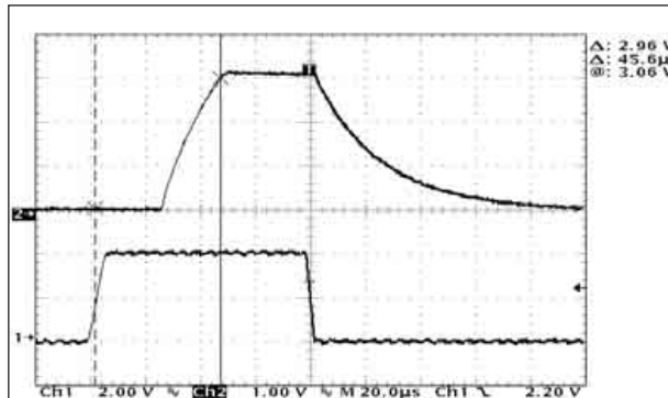
Turn-on Characteristic ( V_{IN} = 4V , I_{OUT} = 100mA )
