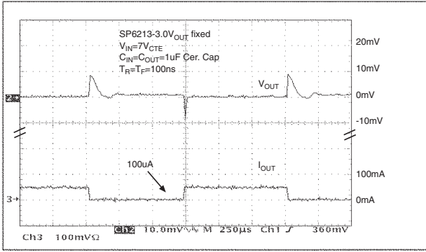
Load Transient Response ( V_{IN} = 7V )
