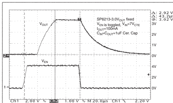
Turn on Time ( V_{IN} = 7V , I_{OUT} = 100mA )
