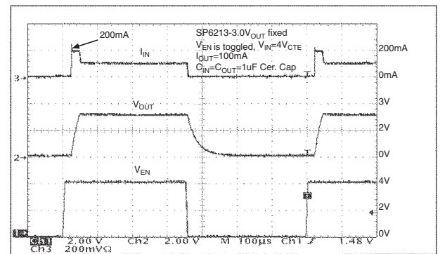
In-Rush Current ( V_{IN} = 4V , I_{OUT} = 100mA )
