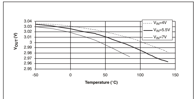
Output Voltage vs. Temperature ( I_{OUT} = 100mA )
