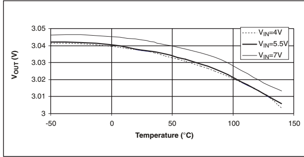
Output Voltage vs. Temperature ( I_{OUT} = 0.1mA )
