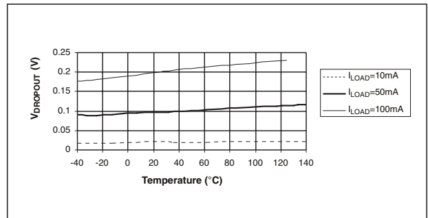
Dropout Voltage vs. Temperature
