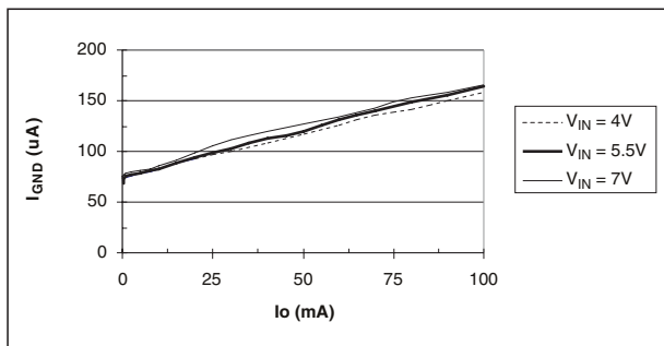
Ground Current vs. Output Current
