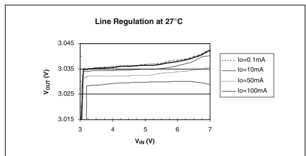
Output Voltage vs. Input Voltage
