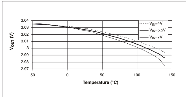
Output Voltage vs. Temperature ( I_{OUT} = 50mA )
