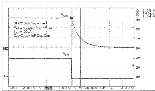
Turn off Time ( V_{IN}=4V , I_{OUT}=100\mu A )
