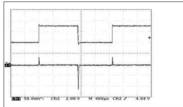
Line Transient Response ( V_{IN}=7V , I_{OUT}=10\mu A )
