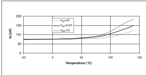
Quiescent Current vs. Temperature ( I_{OUT} = 0A )
