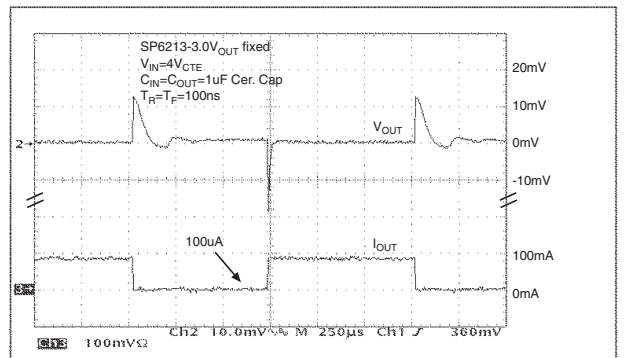
Load Transient Response ( V_{IN} = 4V )
