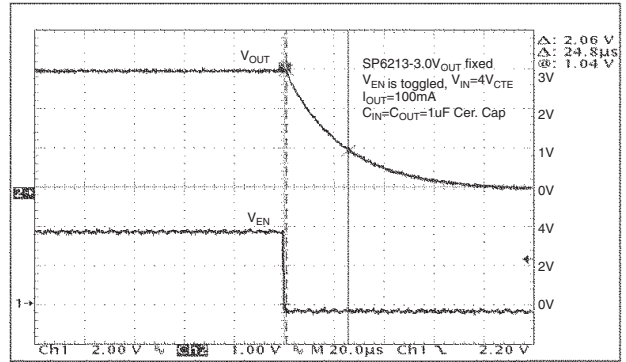
Turn off Time ( V_{IN} = 4V , I_{OUT} = 100mA )
