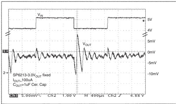
Line Transient Response ( V_{IN}=4V , I_{OUT}=100\mu A )
