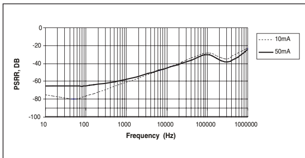
Power Supply Rejection Ratio, V_o=3V
