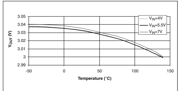
Output Voltage vs. Temperature ( I_{OUT} = 10mA )
