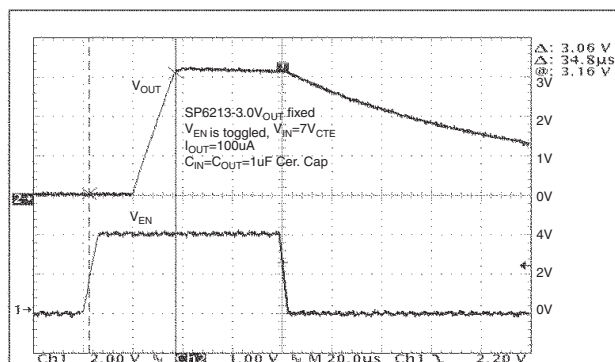
Turn-on Characteristic ( V_{IN} = 7V , I_{OUT} = 100\mu A )
