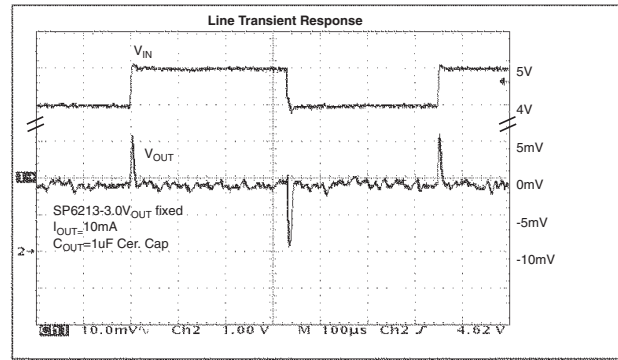
Line Transient Response ( V_{IN}=4V , I_{OUT}=10mA )
