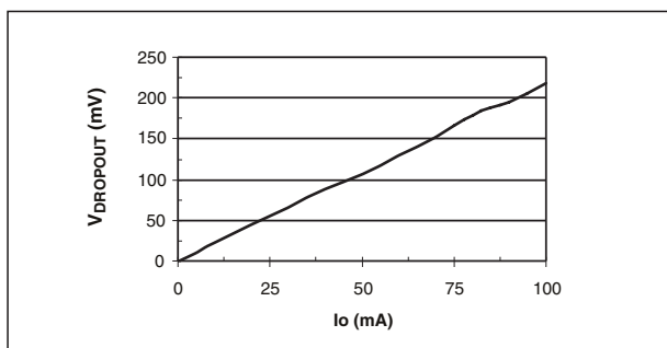
Dropout Voltage vs. Output Current
