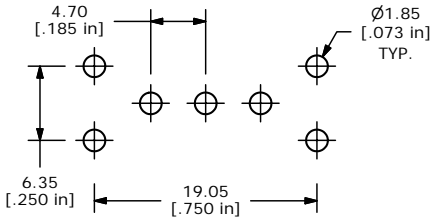
P.C. MOUNTING
